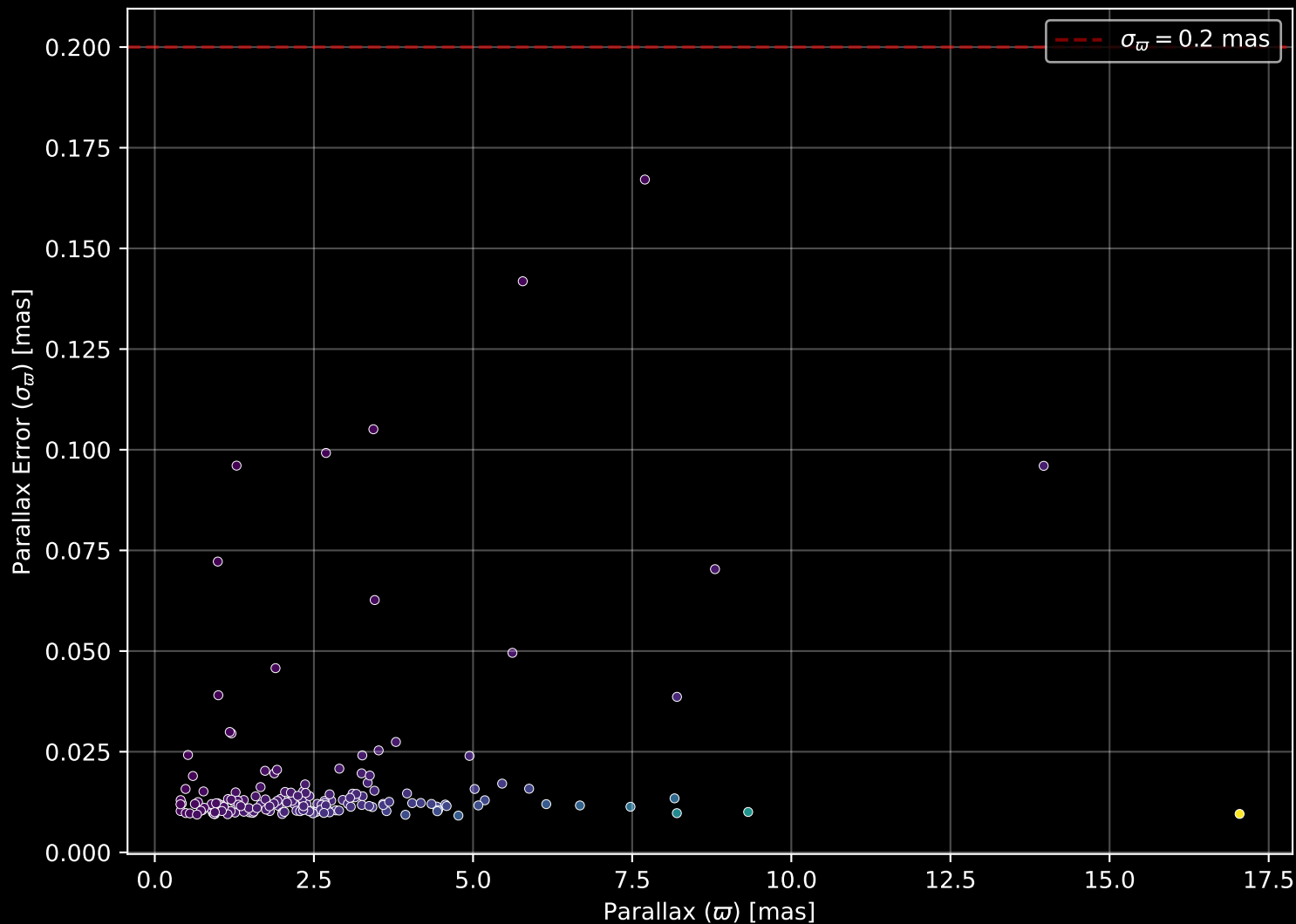
GALAH DR4 Field: [7121] Parallax Quality (n= 168)
