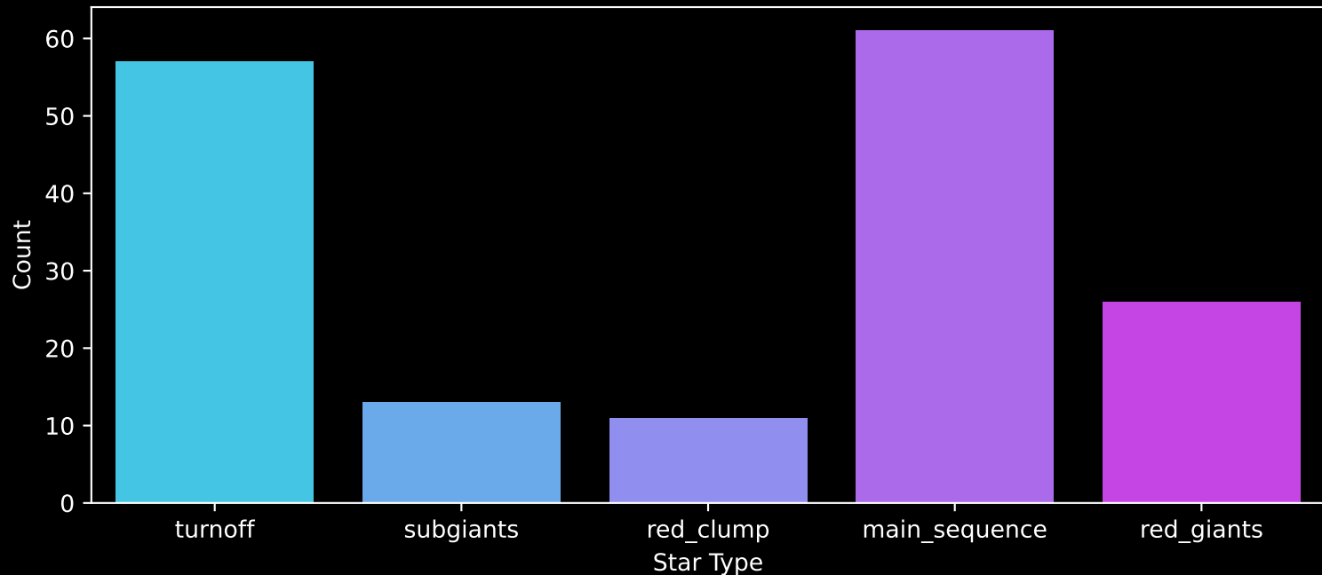
GALAH DR4 Field: [7121] Count plot of Star Type
