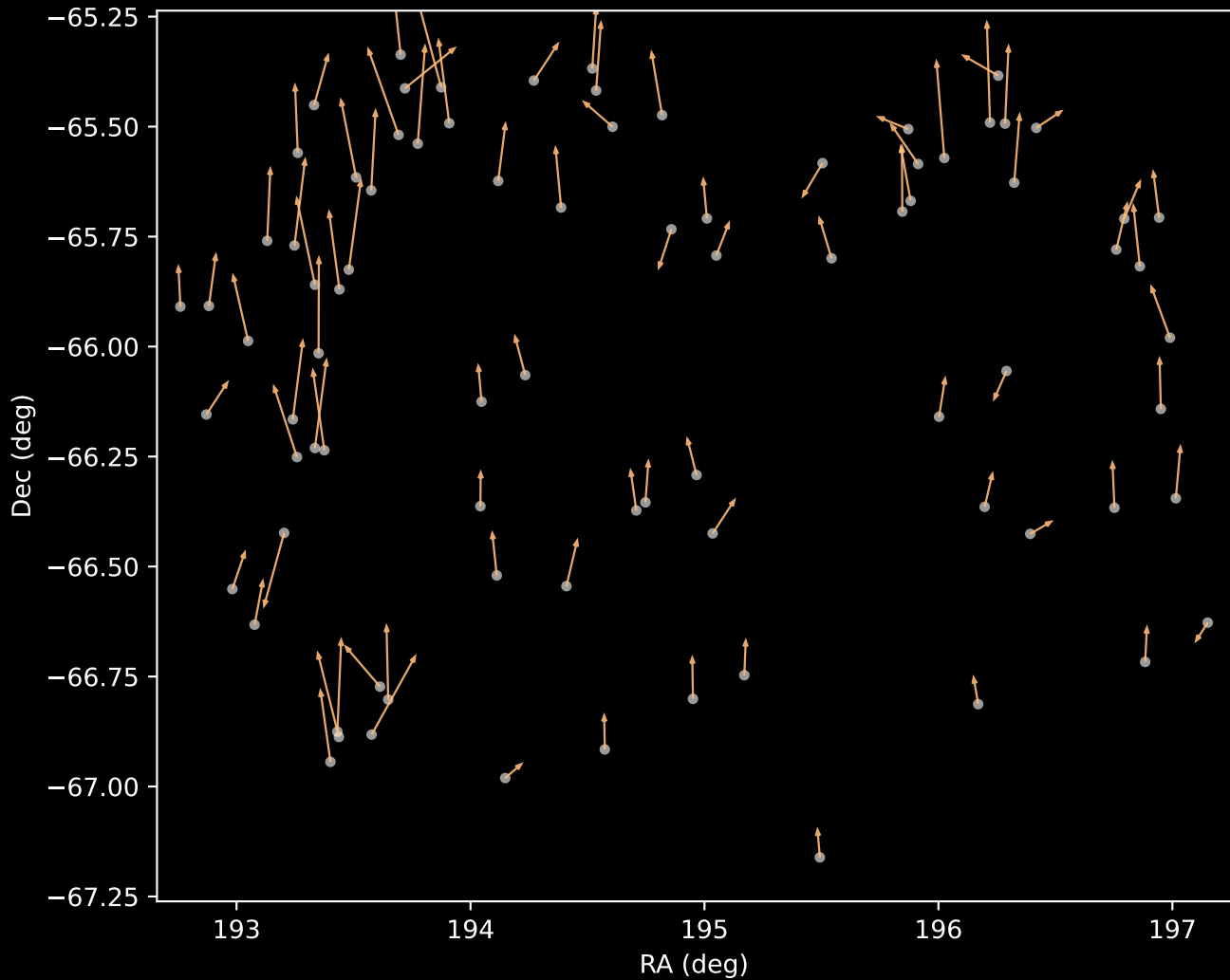
GALAH DR4 Cluster 3 Proper Motion Vectors (n=84)
