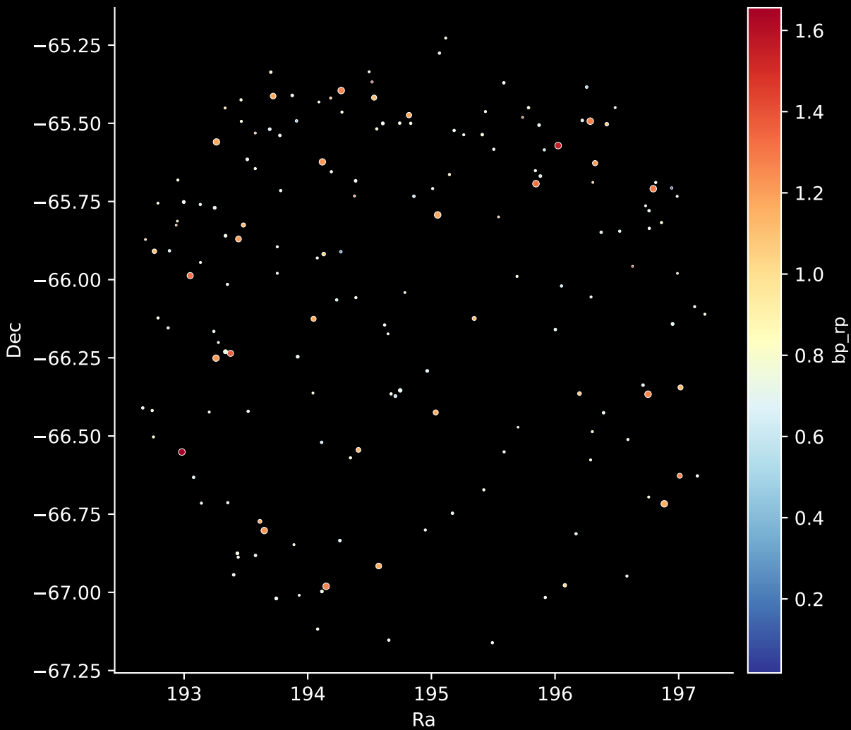
GALAH DR4 Field: [7121] Stars: 168
