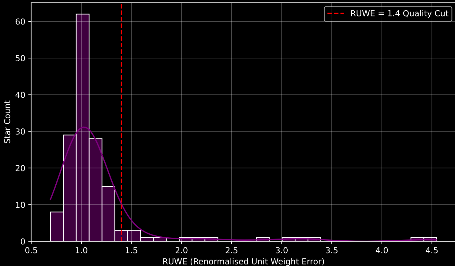
GALAH DR4 Field [7121] RUWE Distribution (n= 159)
