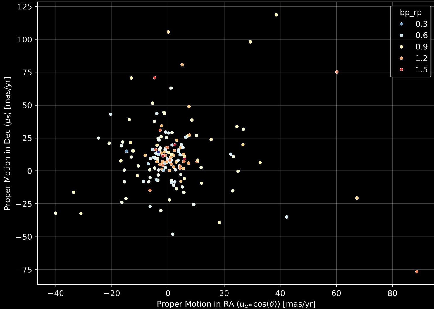
GALAH DR4 Field: [7121] Proper Motion Diagram (n= 168)
