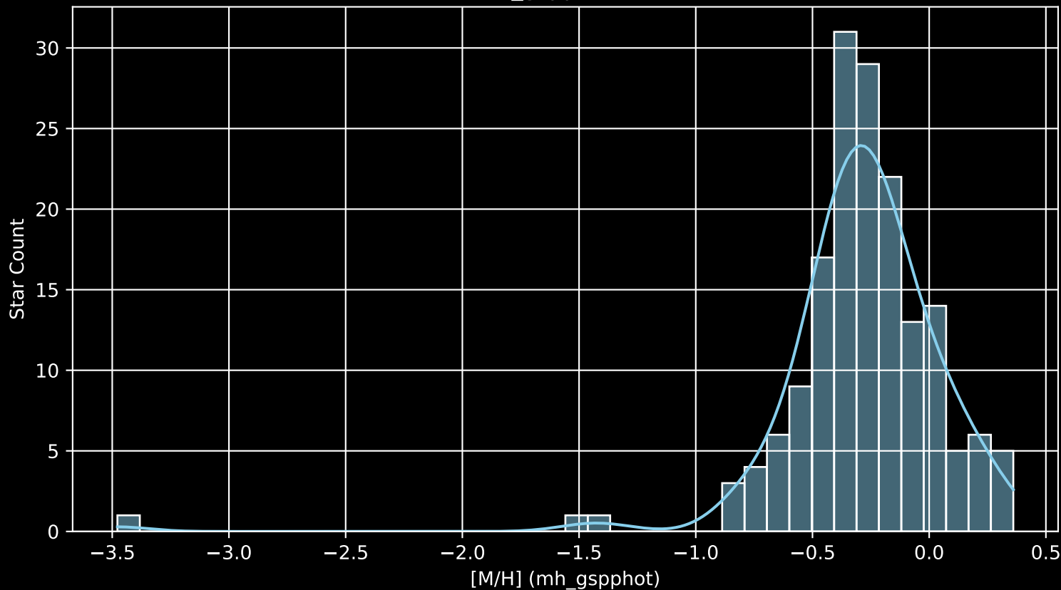
GALAH DR4 Field: [7121] [M/H] (mh_gspphot) (n= 167)
